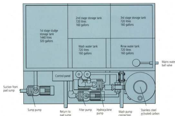
Plan view of Integra type reclaim system. Covers omitted for clarity. 2400 mm x 1800 mm x 1500 mm high (plus 800 mm for carbon removal)
