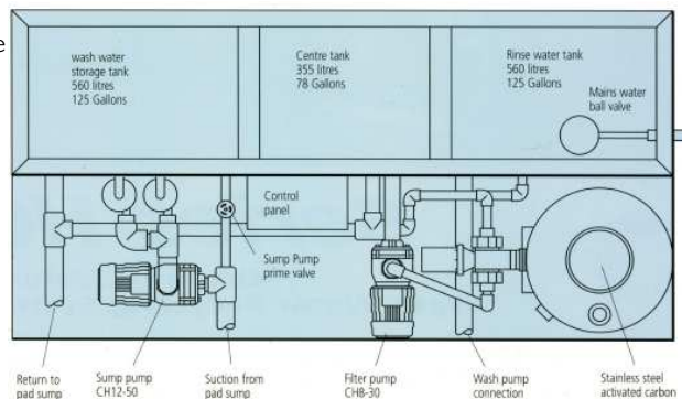
Plan view of HC reclaim system Covers omitted for clarity 2400 mm x 1200 mm x 1500 mm high (plus 800 mm for carbon removal)
